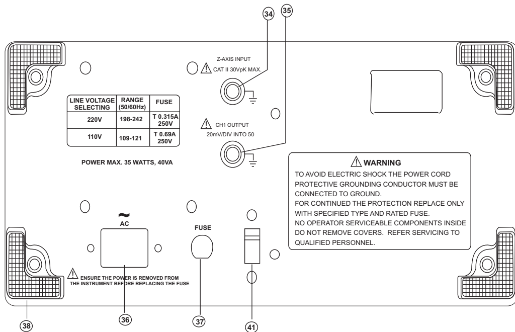
Figure 4-1 MODEL KM-20-10:20MHz
