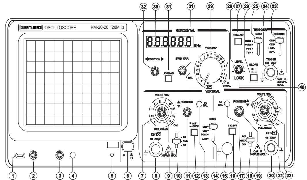
Figure 4-1 MODEL KM 20-20 : 20MHz
